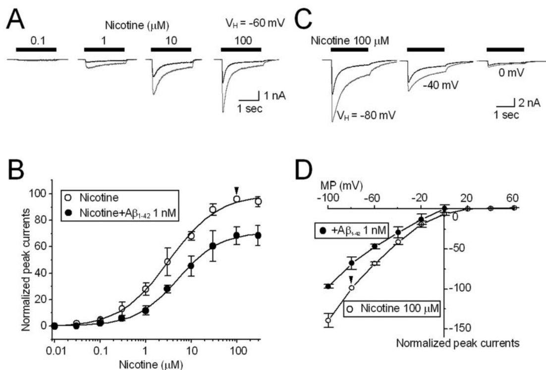
FIG. 4. \text{A}\beta_{1-42} inhibits human \alpha 4\beta 2 -nAChR-mediated currents in a non-competitive and voltage-independent manner. A , individual whole cell current traces for responses to nicotine at the indicated concentrations alone (higher amplitude traces) or in the presence of 1 nM \text{A}\beta_{1-42} (smaller amplitude traces). B , results of replicate studies (as in A ) fit to the logistic equation indicate a downward shift reflecting reduction of maximal current response in the agonist dose-response profile in the presence of \text{A}\beta_{1-42} , but without a change in apparent \text{EC}_{50} for agonist, characteristic of non-competitive inhibition. All symbols were normalized to the peak current induced by 100 \mu\text{M} nicotine (marked by the arrowhead), and each symbol is the average from 10 cells for nicotine, and 5 cells for nicotine plus 1 nM \text{A}\beta_{1-42} . C , representative whole cell current traces in response to 100 \mu\text{M} nicotine alone (higher amplitude traces) or in the presence of 1 nM \text{A}\beta_{1-42} (lower amplitude traces) at different holding potentials as indicated. D , plots of whole cell peak current amplitude as a function of holding potentials. All symbols were normalized to nicotine-induced peak current at a V_H of -80 mV (marked by the arrowhead) and are averages of recordings from 5 to 6 cells. Vertical bars indicate standard errors.
